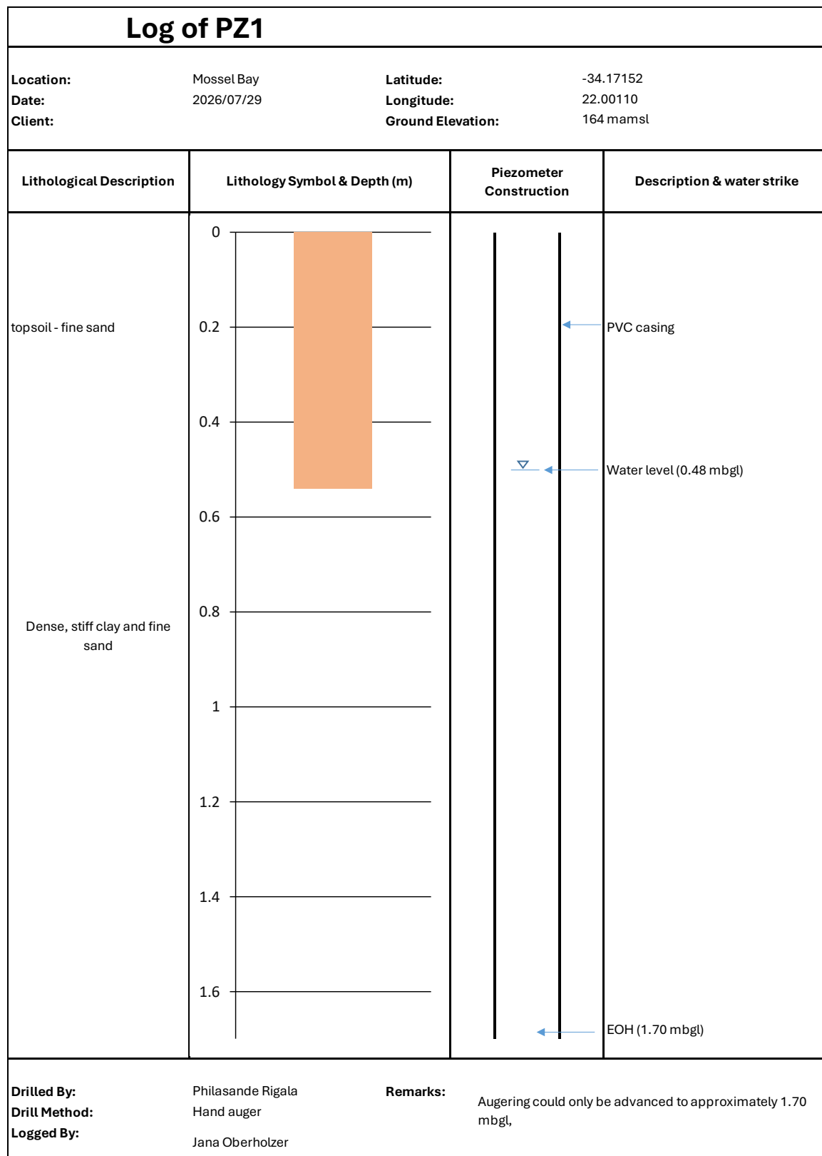
Figure 5: Lithological log of PZ1.
